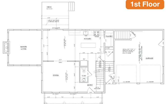
1st Floor
